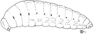
Fig. 91. Vespa macutata Kirby.
